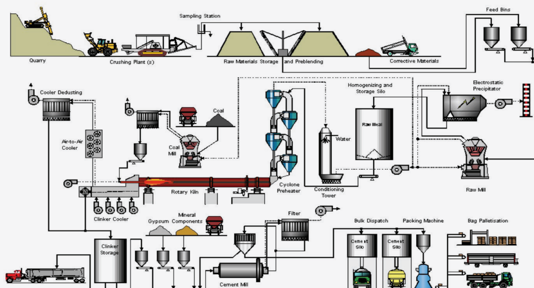
Figure 1. Diagram for Cement Manufacturing Preheater Process
